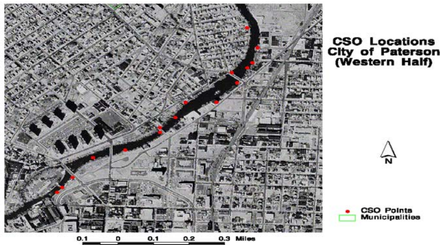
Figure 3.25 CSO Locations in the City of Paterson (NJDEP, 2010)
